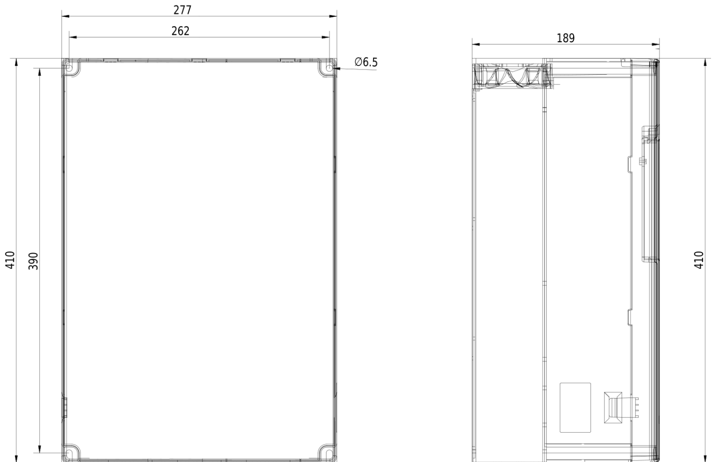
Dimensional drawing V810 - 37kW 4T0370
