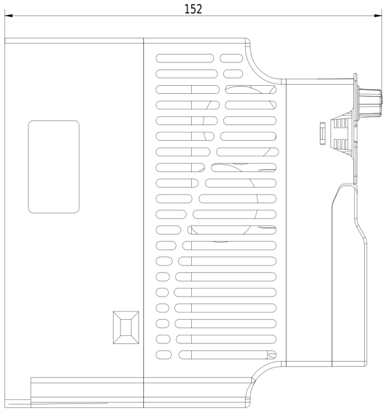
Dimensional drawing V800 - 0,4kW 2S0004
