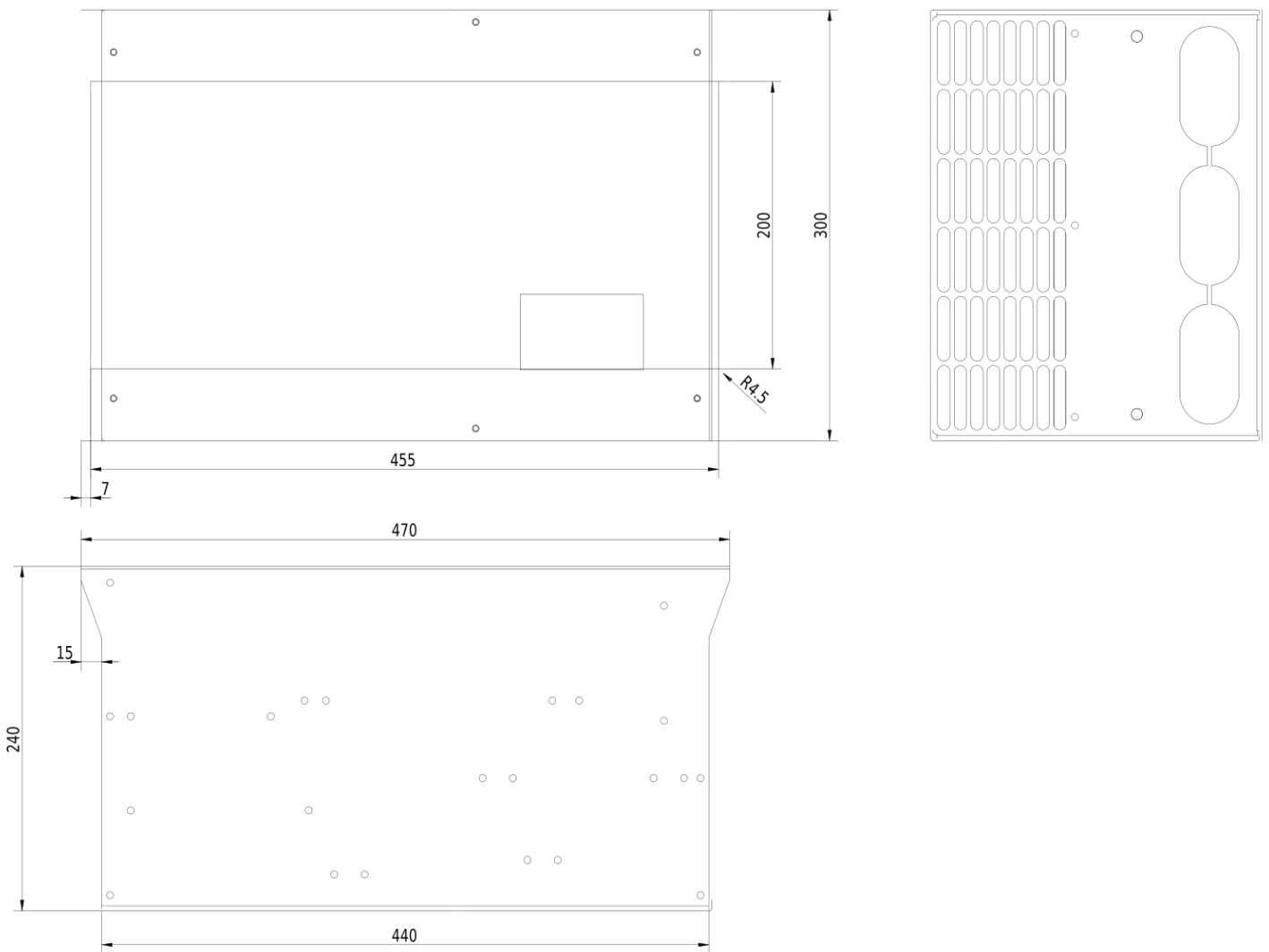
Dimensional drawing V900 - 75kW 4T0750
